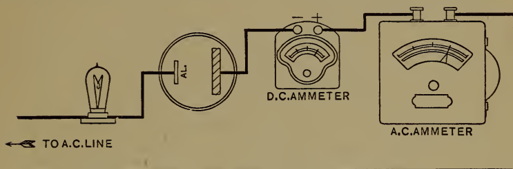
FIG. 20.—TESTING A NODON VALVE WITH ALTERNATING CURRENT.
